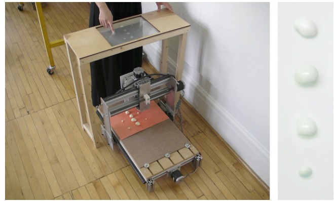
Figure 2. Shaper , a prototype device for interactive fabrication (left) using expanding polyurethane foam (right).
