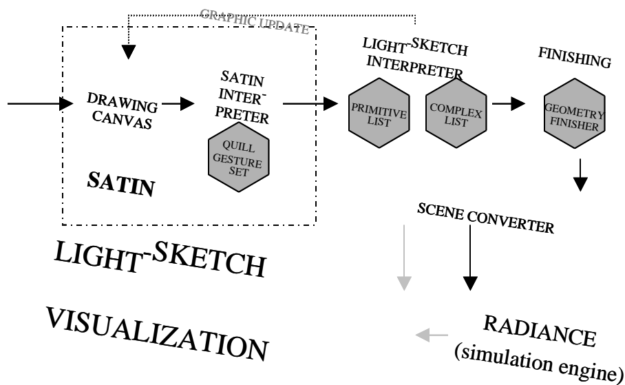
Figure 7. The main modules of LightSketch and its relationship to the simulation engine and visualization routines. Gray arrows are under development.
