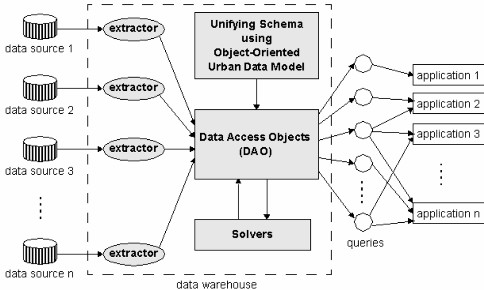
Figure 4. The overall architecture of an urban data warehouse
