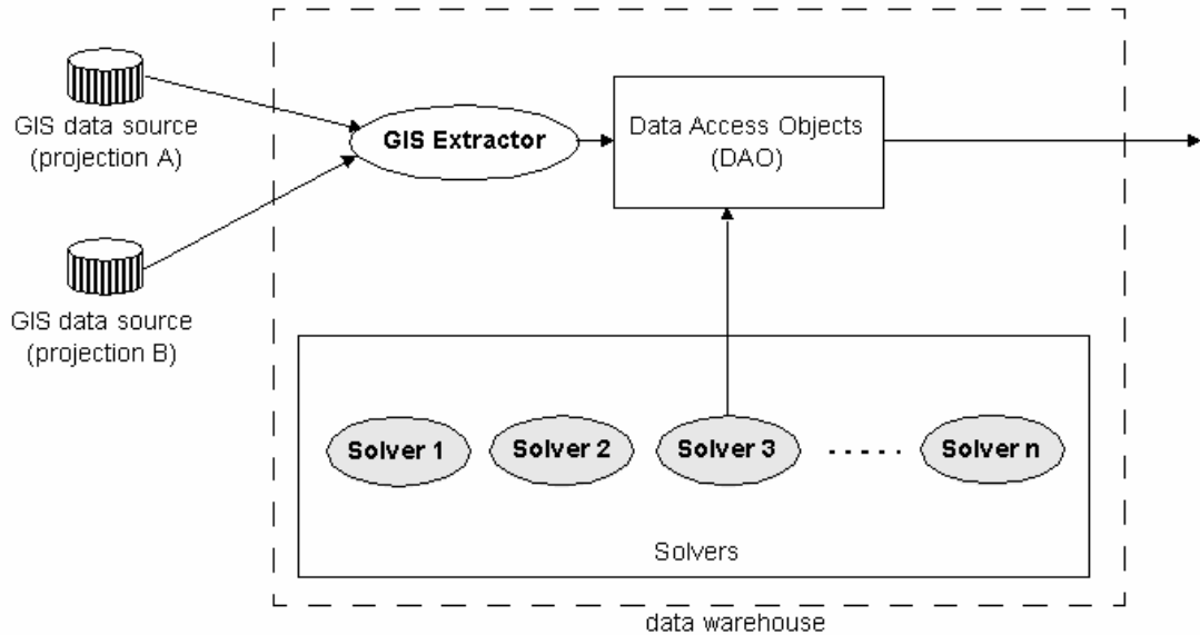
Figure 6. Solvers in the data warehouse
