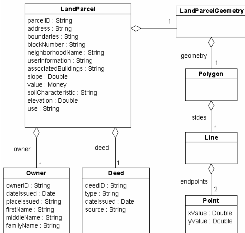
Figure 1. LandParcel Class
