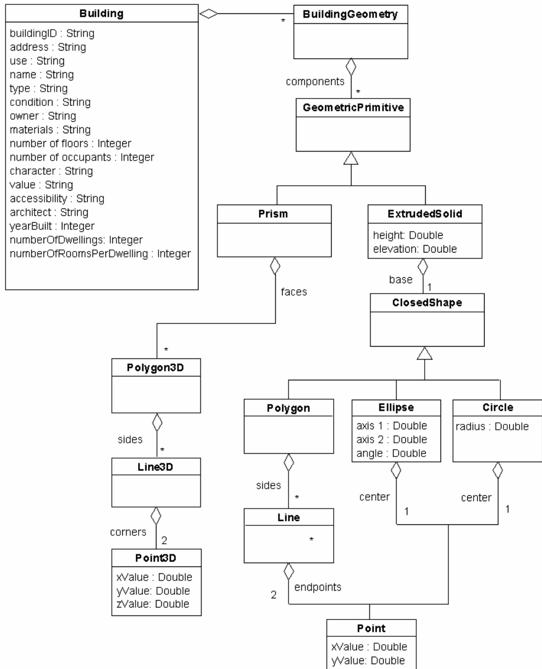
Figure 2. Building Class
