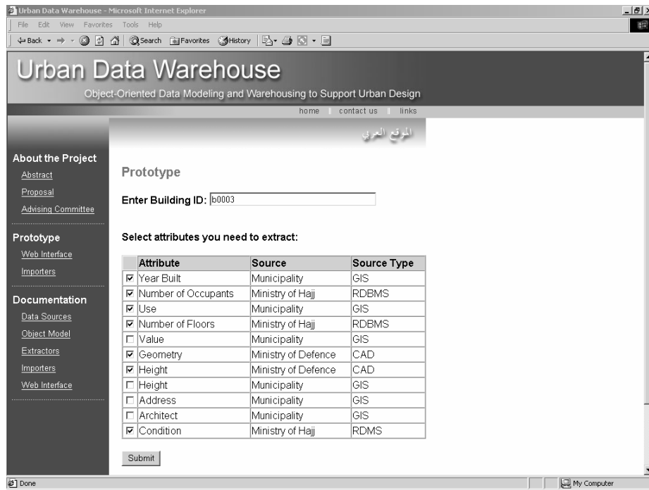
Figure 7. Web Interface to the data warehouse
