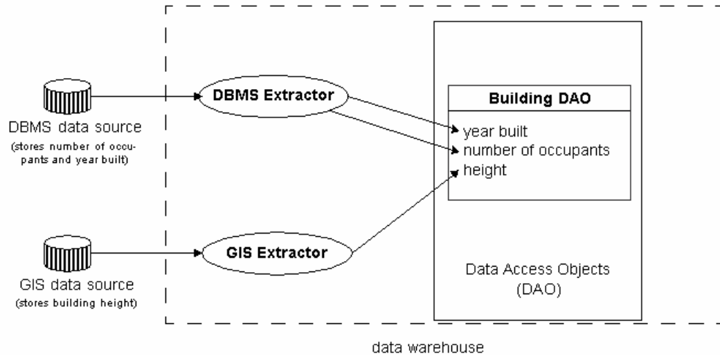
Figure 5. Interactions between data sources, Extractors, and DAOs
