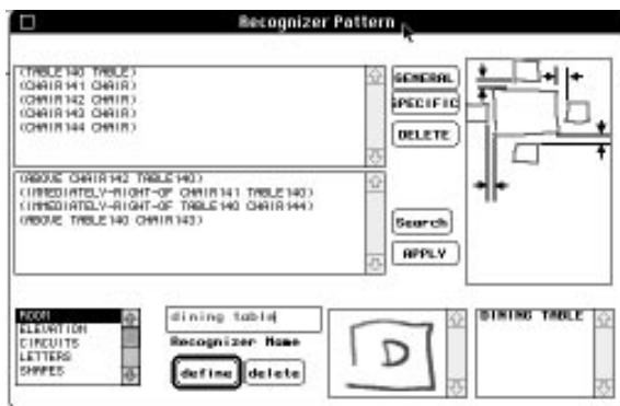
Figure 4. Defining a configuration by example: The Napkin shows relations, the user edits them.
